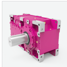
B.01 With solid output shaft
