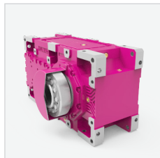
B.05 With shrink disk
